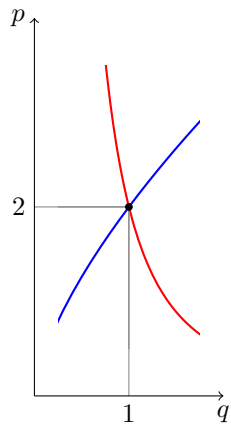
Figure 1: Elastic Equilibrium
