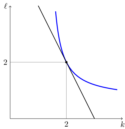
Figure 3: CES Choice
