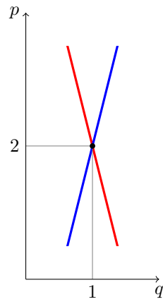
Figure 2: Linear Equilibrium
